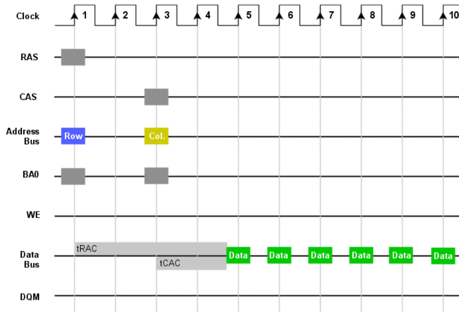
SDRAM Read
